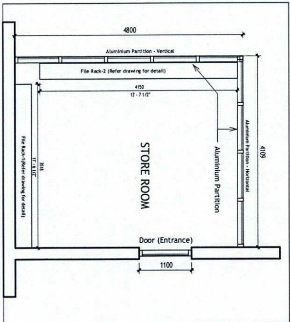
STORE ROOM PLAN
