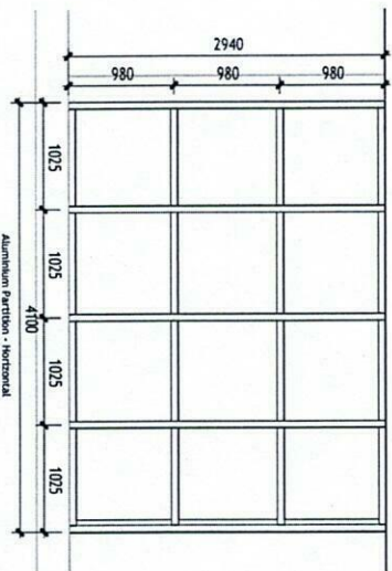
ALUMINIUM PARTITION - HORIZONTAL
