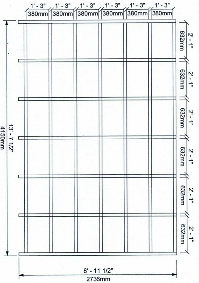
1 FRONT VIEW Cross-sectional Dimension of plank = 2"x1'-2" (51mm x 350mm) Material used = Broad Leaf wood
