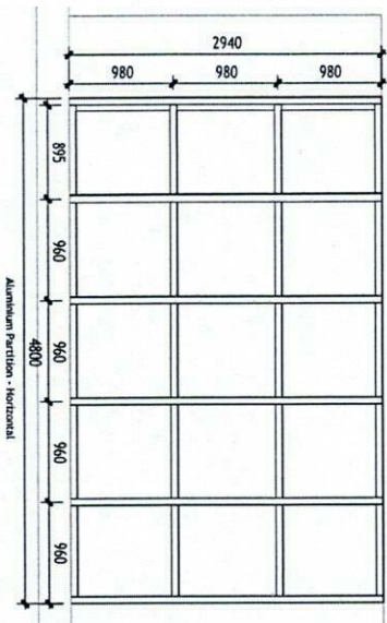
ALUMINIUM PARTITION - VERTICAL
