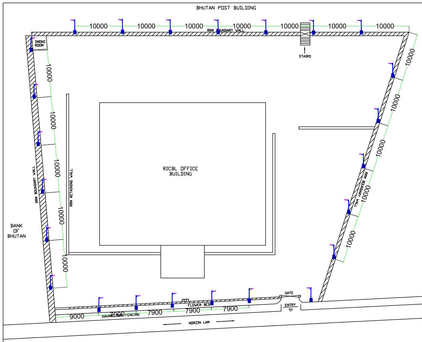
SITE PLAN WITH POLE LAYOUT
